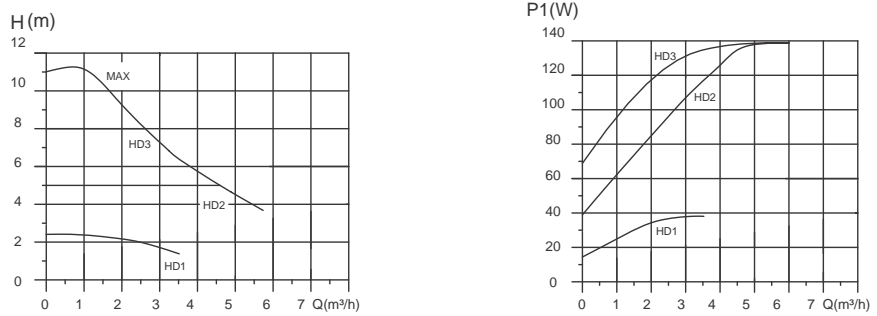
RCE 25-11 Series Performance Chart (Constant Pressure)
